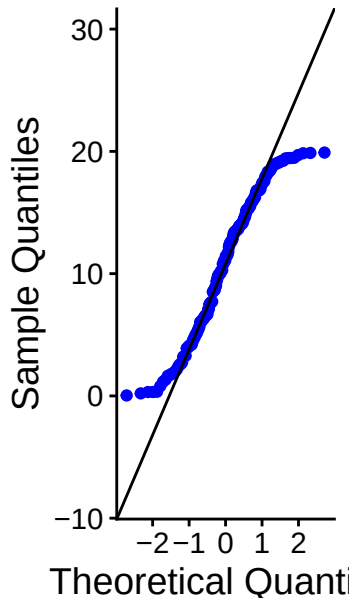
Q-Q plot
