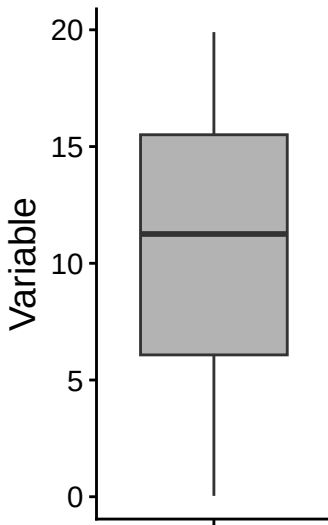
Box Plot
